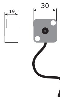
MIC
